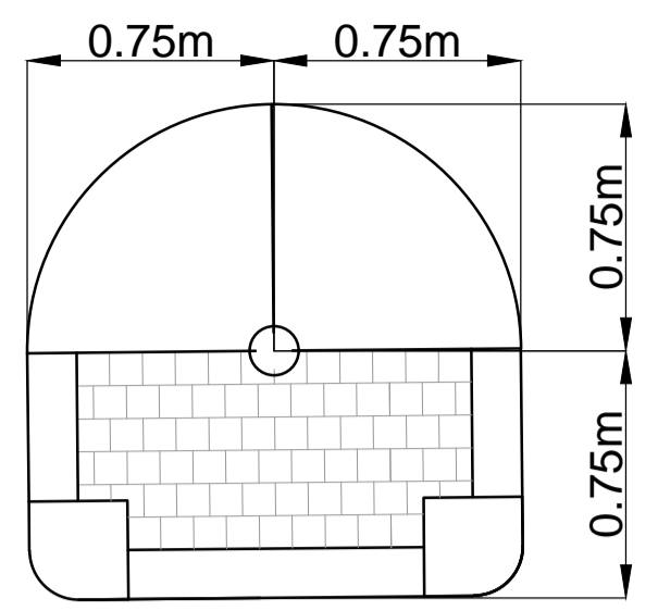
Traffic Island Signal Pole Detail - 1:25
